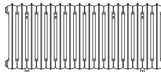
560 x 1344 16 sections
