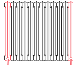
920 x 1016 12 sections (2+10)
