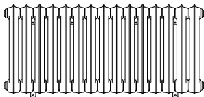
560 x 1262 15 sections
