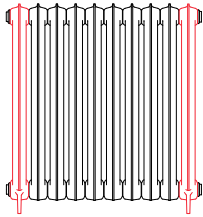
920 x 852 10 sections (2+8)
