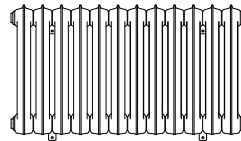
560 x 1016 12 sections
